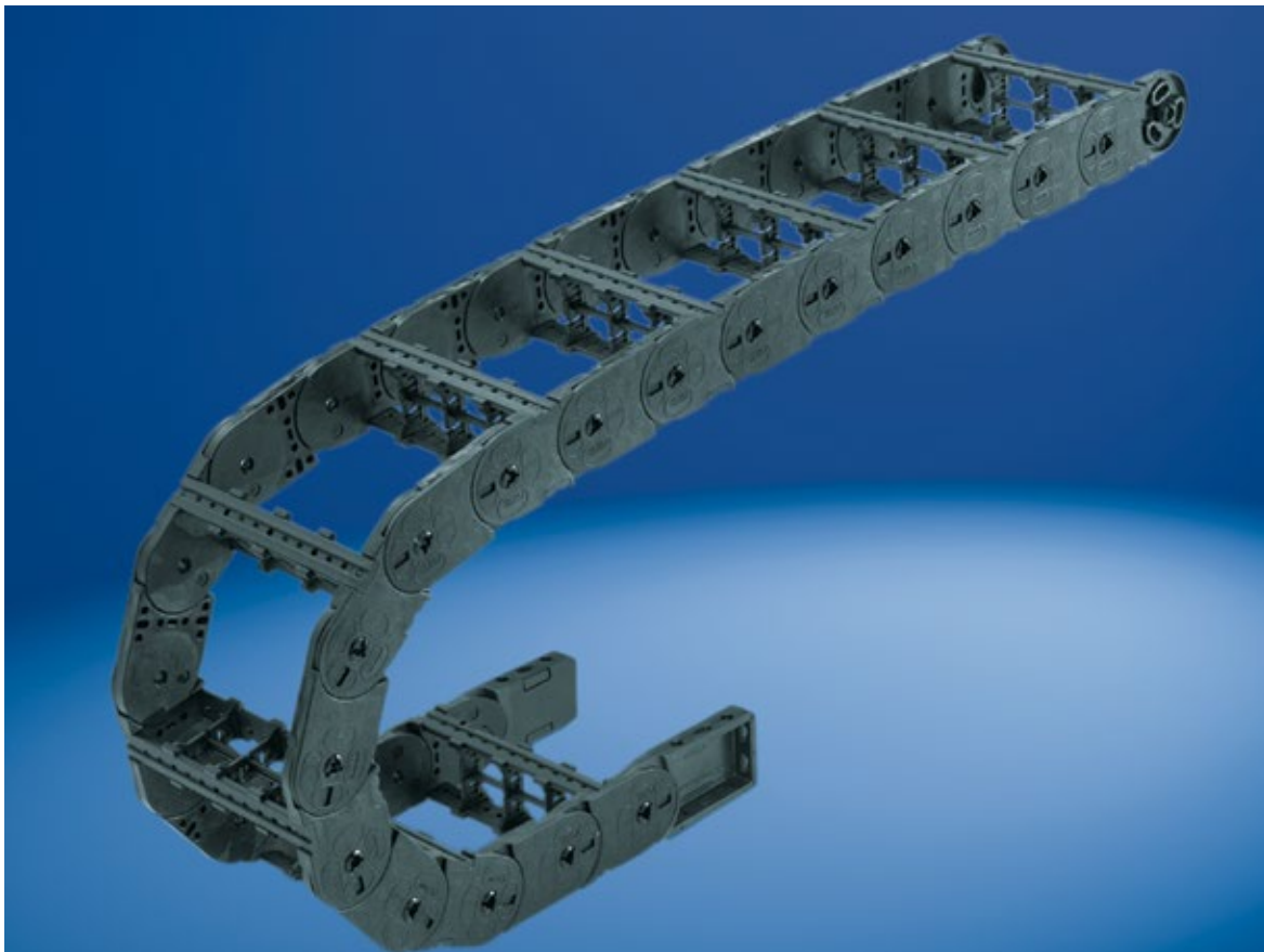
The robust cable carrier KE0900 is suitable even for high additional loads and features an encapsulated stroke system which is resistant to dirt
